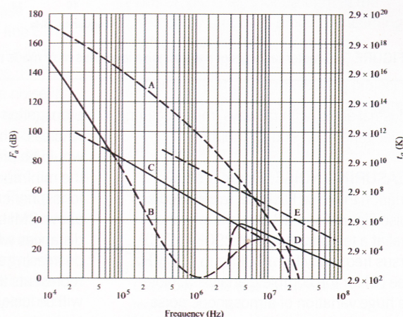
FIGURE 1: Noise Figure in dB above the reference noise temperature, 290K (17°C). A – atmospheric noise, value exceeded 0.5% of the time. B – atmospheric noise, value exceeded 99.5% of the time. C – man-made noise, quiet receiving site. D – Galactic noise. E – median city area man-made noise. The solid line indicates the minimum noise level expected. (Source: ITU-R Recommendation P.372-10 (10/2009), used with permission).
