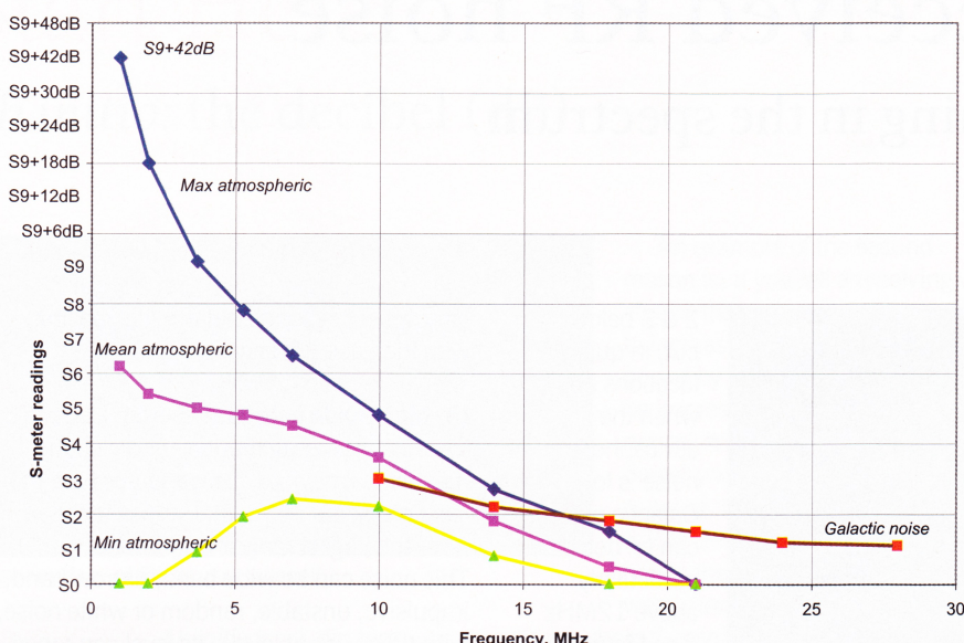
FIGURE 2: S-meter readings of natural noise level.
